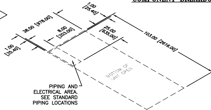
FRAME DIMENSIONS
