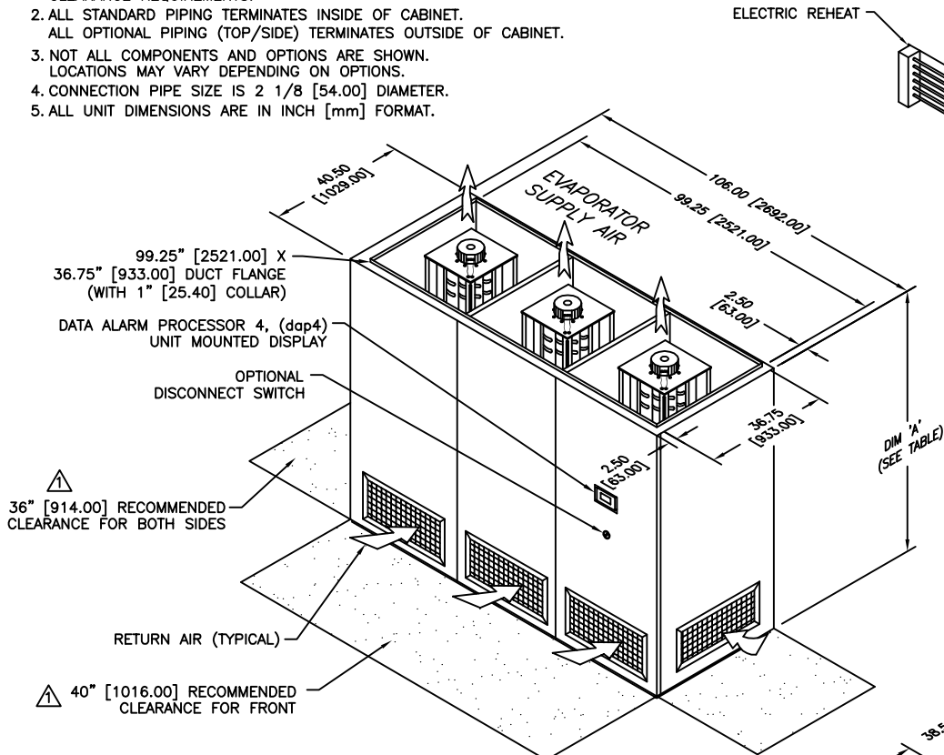
DIMENSIONAL DATA
