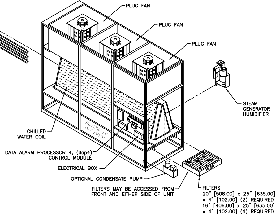
COMPONENT BREAKDOWN
