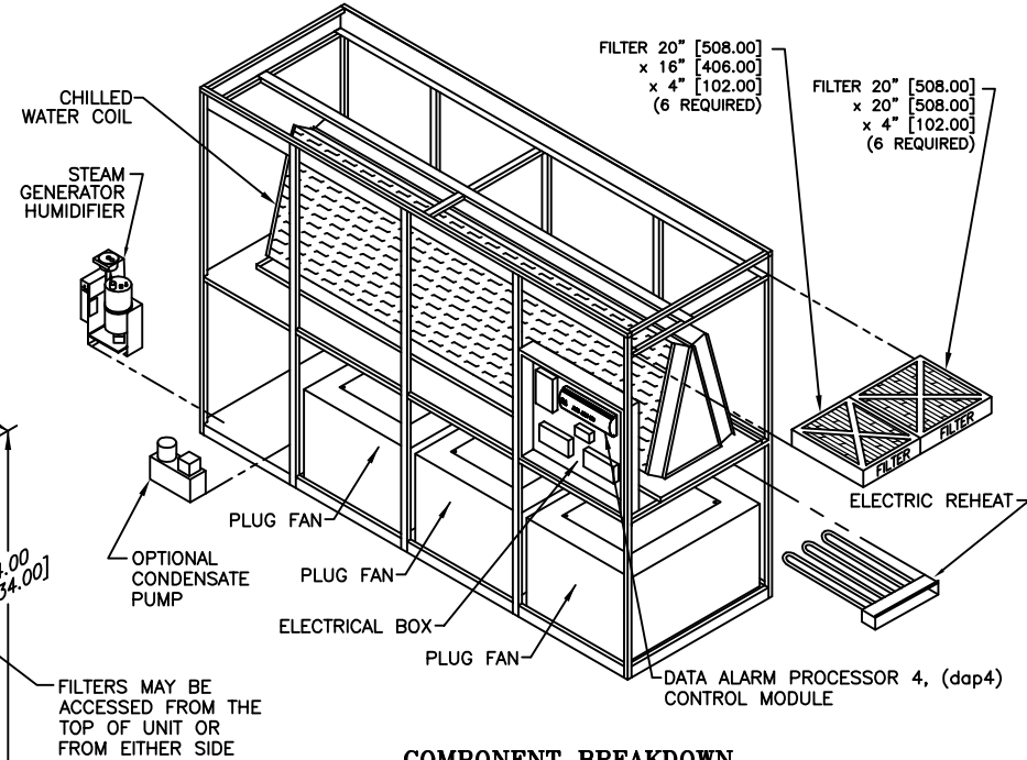
COMPONENT BREAKDOWN
