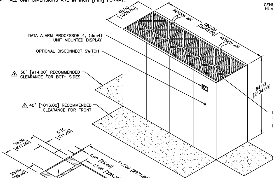
DIMENSIONAL DATA
