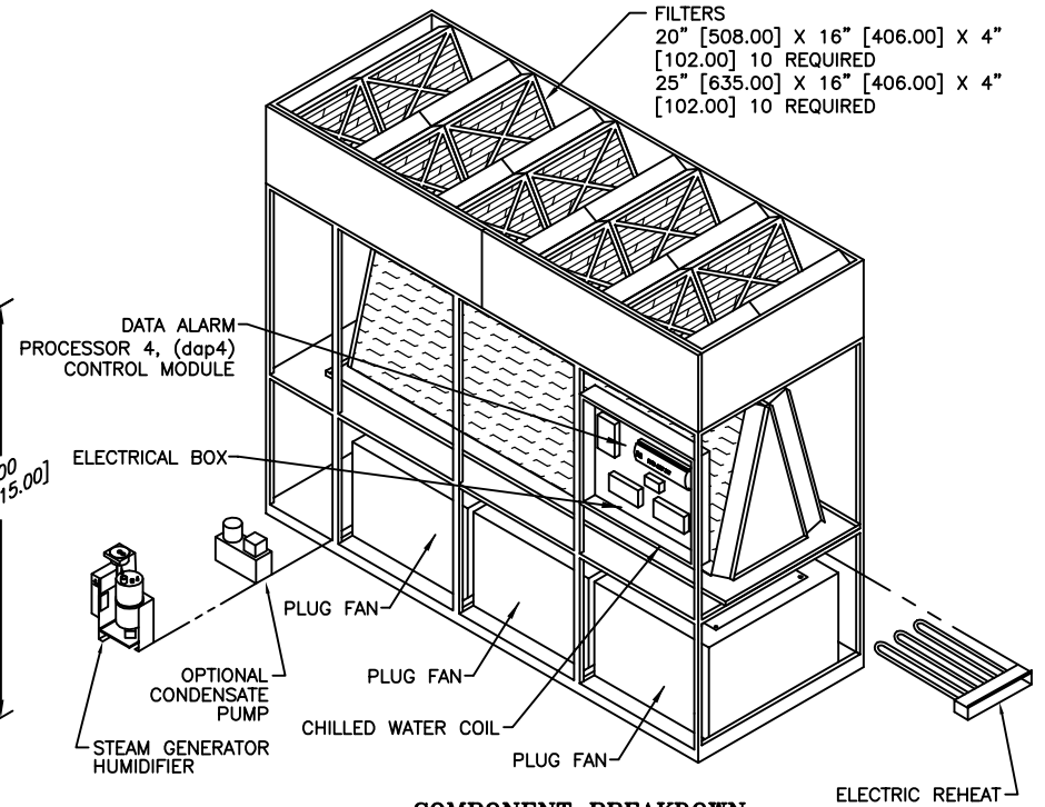
COMPONENT BREAKDOWN
