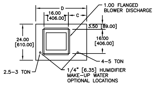
DETAIL -C- EVAPORATOR SUPPLY AIR
