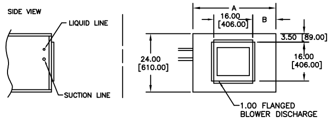
DETAIL -A- CONDENSING DISCHARGE AIR
