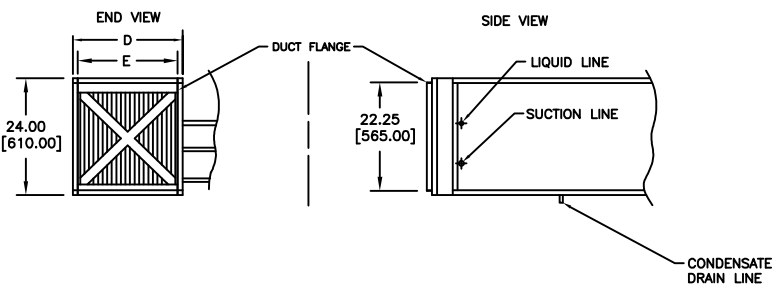
DETAIL -B- EVAPORATOR RETURN AIR
