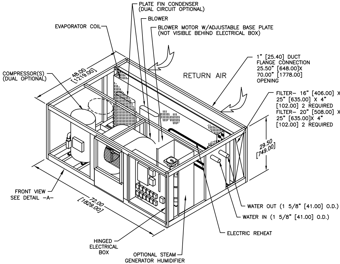
WATER COOLED INDOOR EVAPORATOR (SHOWN WITHOUT PANELS)
