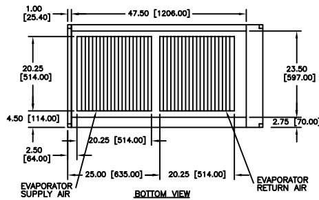
DETAIL -B- EVAPORATOR SUPPLY & RETURN AIR
