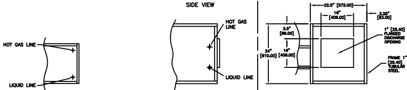
DETAIL -D- CONDENSER DISCHARGE AIR
