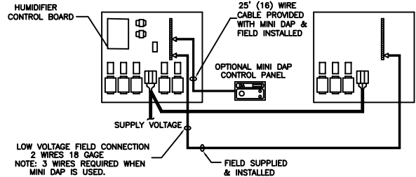
DETAIL -E- EVAPORATOR SECTION ELECTRICAL BOX
