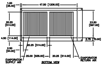
DETAIL -B- EVAPORATOR SUPPLY & RETURN AIR
