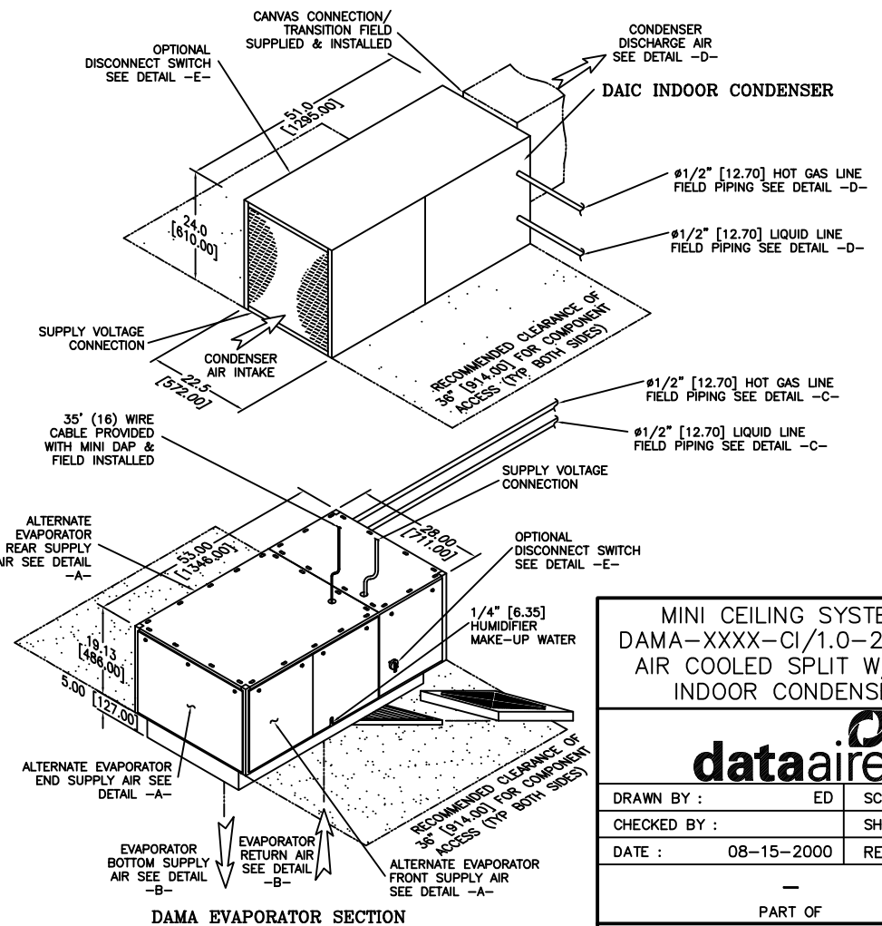
DAMA EVAPORATOR SECTION
