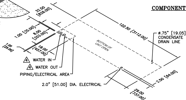
FOOTPRINT LAYOUT (PIPING & ELECTRICAL AREA REFERENCE)
