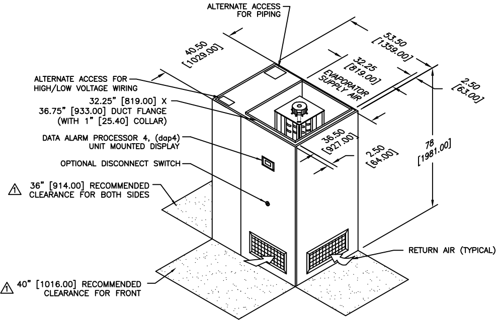
DIMENSIONAL DATA
