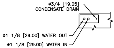
WATER/GLYCOL COOLED
