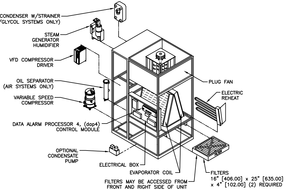
COMPONENT BREAKDOWN
