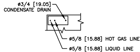
AIR COOLED
