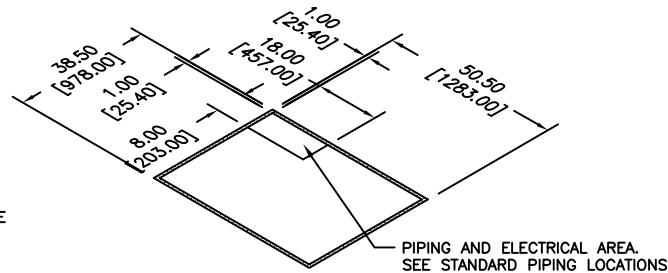
FRAME DIMENSIONS
