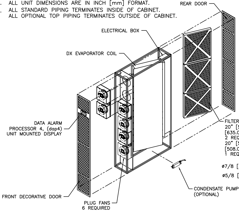
COMPONENT BREAKDOWN
