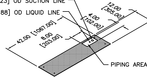
BOTTOM PANEL LAYOUT DIMENSIONS (PIPING AREA REFERENCE)
