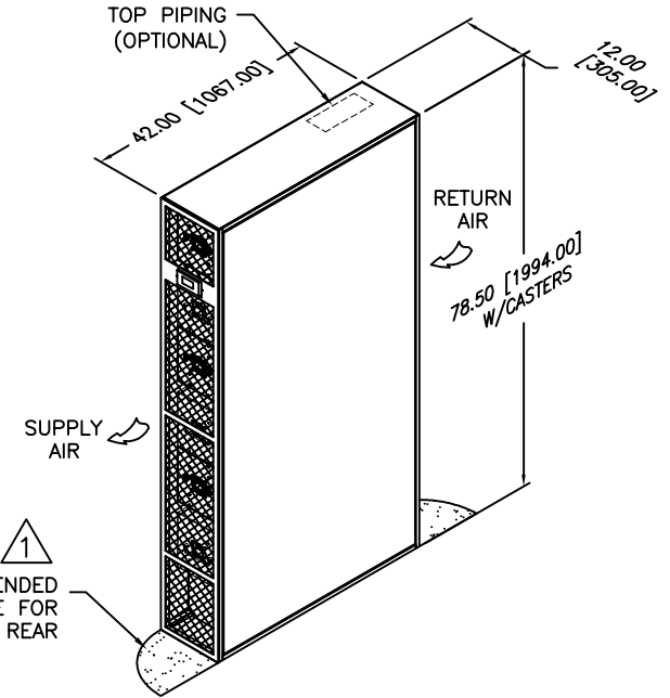
DIMENSIONAL DATA
