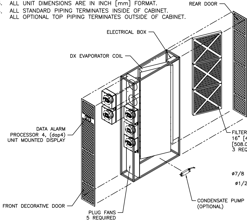
COMPONENT BREAKDOWN
