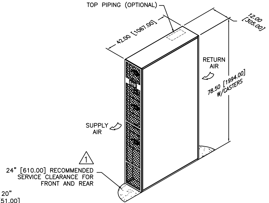
DIMENSIONAL DATA
