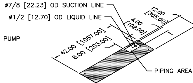
BOTTOM PANEL LAYOUT DIMENSIONS (PIPING AREA REFERENCE)
